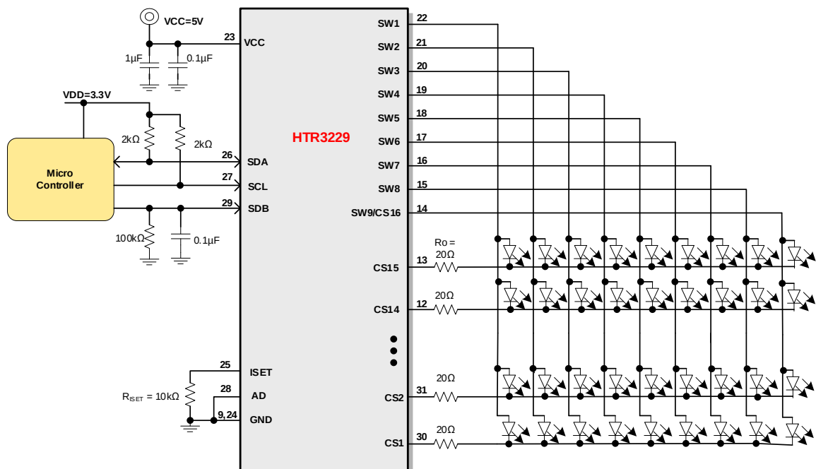
Driving 15×9 LEDs
