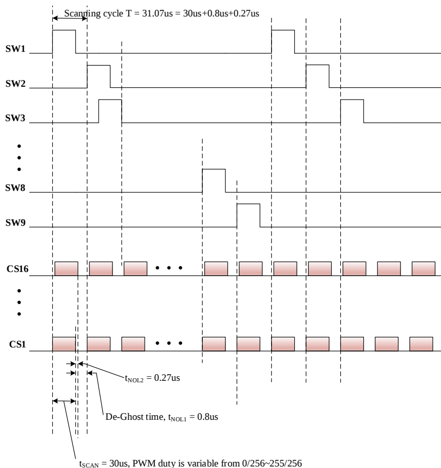
Figure 6 Scanning Timing
