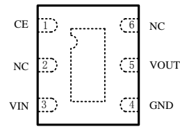
DFN1820-6L (TOP VIEW)
