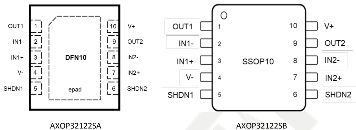
Figure 4 AXOP32122SA/B Pinouts
