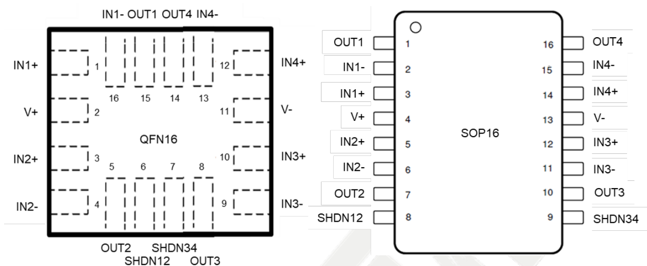
Figure 6 AXOP32124SA/B Pinouts
