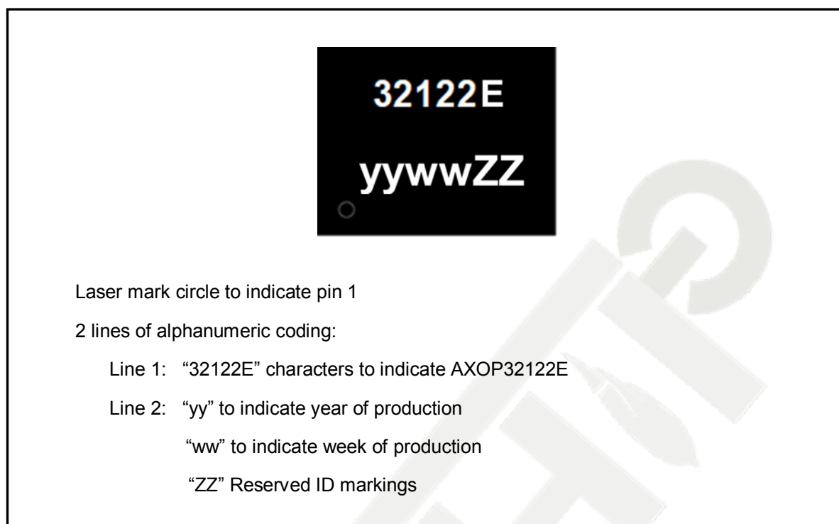
Figure 31 DIP8L Marking Information
