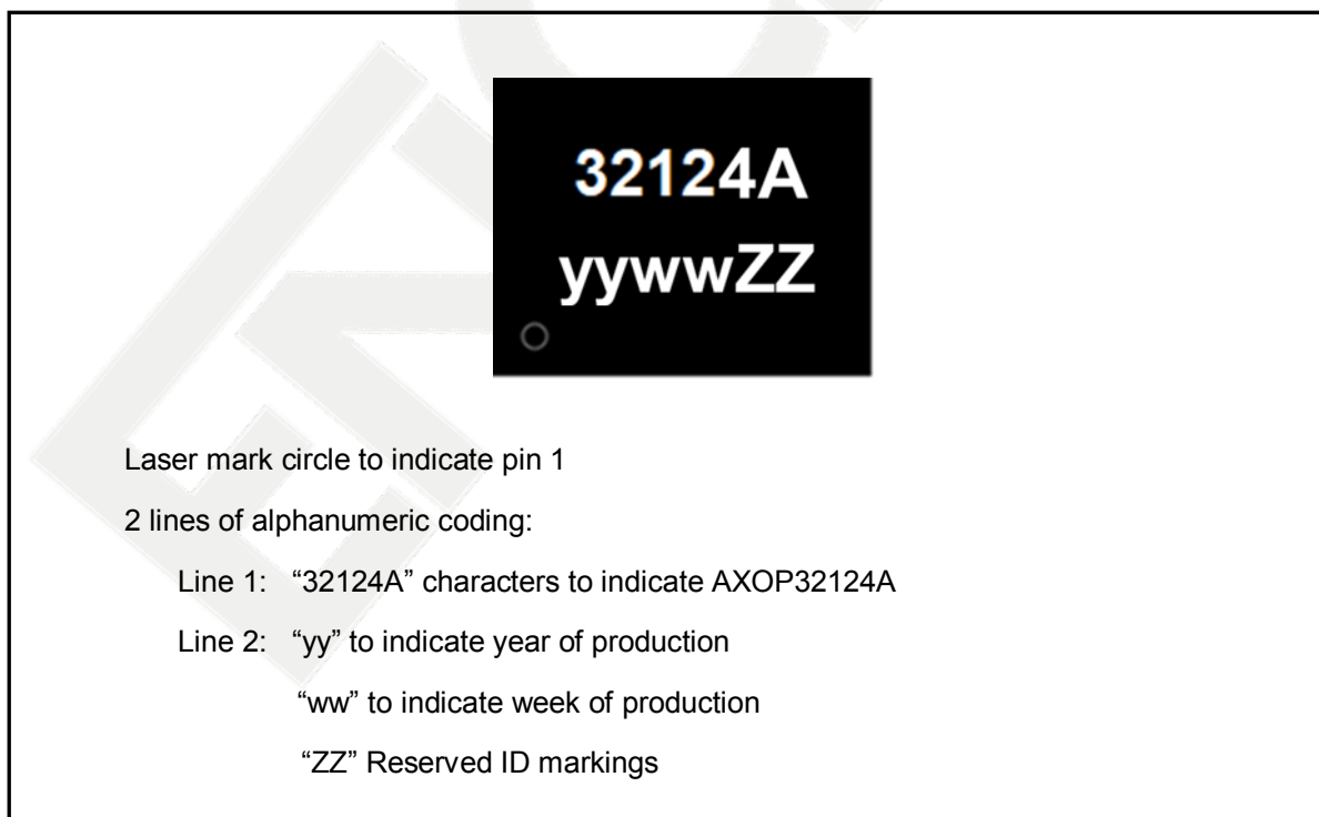
Figure 34 QFN14 Marking Information
