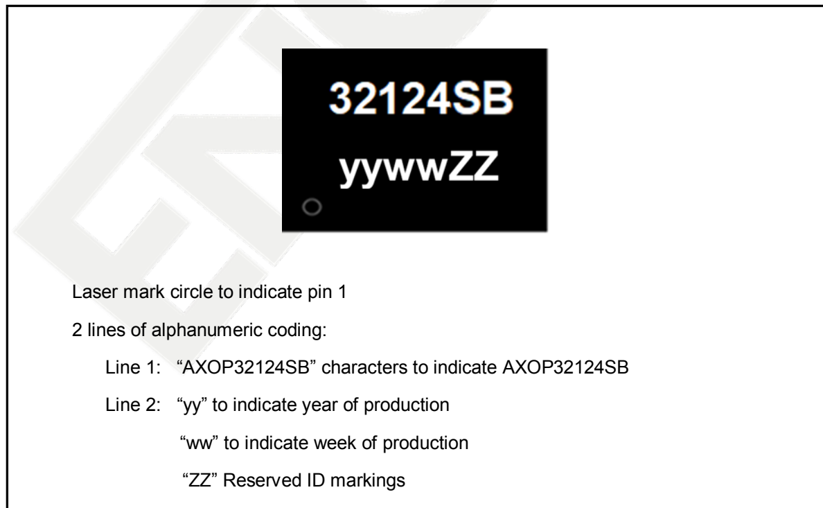
Figure 38 SOP16 Marking Information
