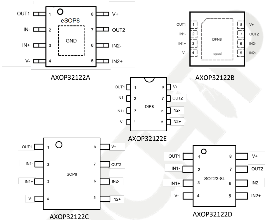
Figure 3 AXOP32122A/B/C/D/E Pinouts
